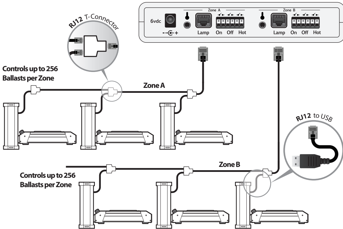
APDPX1 System Connection Drawing
