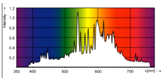
3100k - 315W Lamp (BUcMh31531K)
