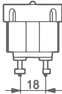
T5 BULB SHAPE WITH PGZ18 LAMP BASE
