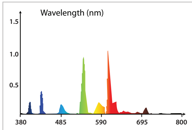
Spectrum for the BLB023-2900k lamp
