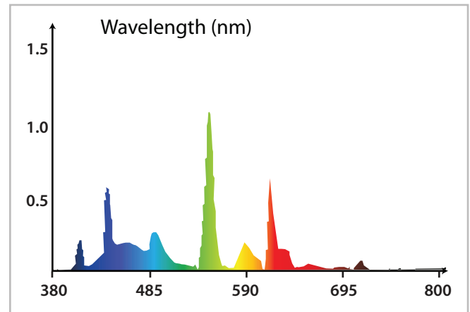
Spectrum for the BLB021-6500k lamp
